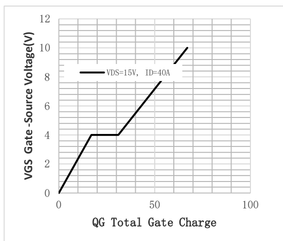
Fig.1 Gate-Charge Characteristics
